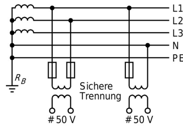
Abb. 22: SELV
